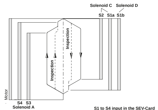
Electrical sequence
