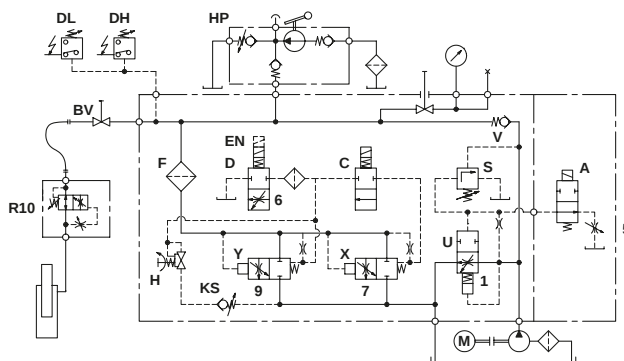
Hydraulic circuit
