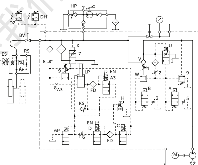
Hydraulic circuit
