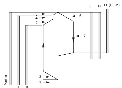
Electrical sequence
